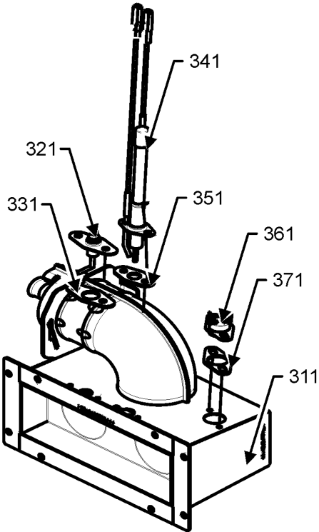
BURNER ASSEMBLY
