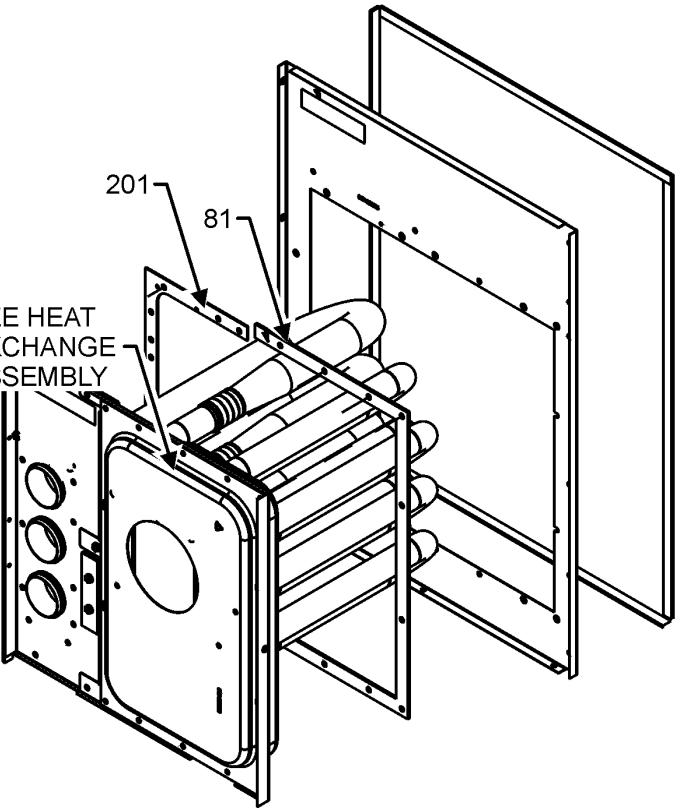
HEAT EXCHANGE ASSEMBLY
