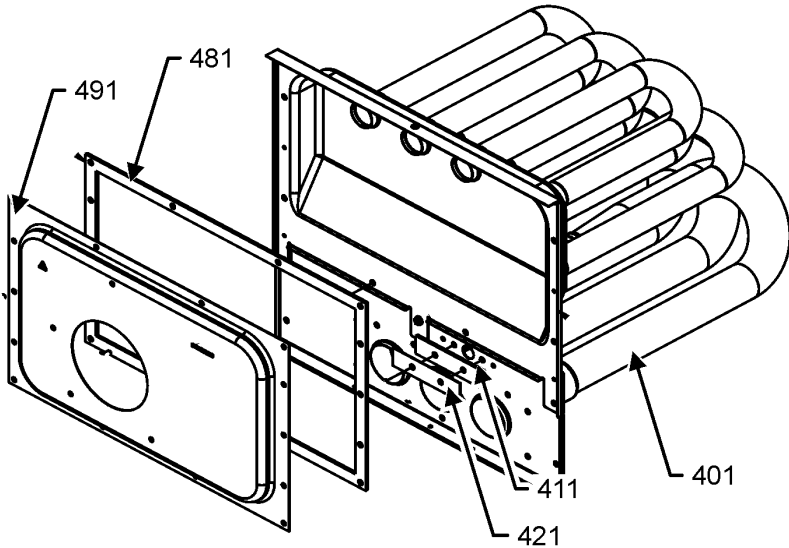
HEAT EXCHANGE ASSEMBLY
