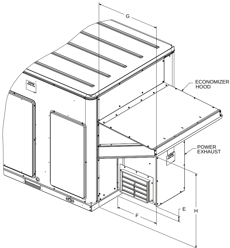
Figure 38. A.0, B.0 and C.0 cabinet – power exhaust with low leak economizer
