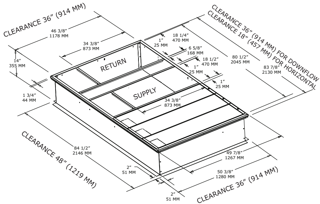
Figure 27. B.O cabinet – roof curb
