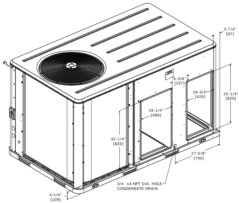
Figure 25. B.0 cabinet – horizontal airflow supply/return
