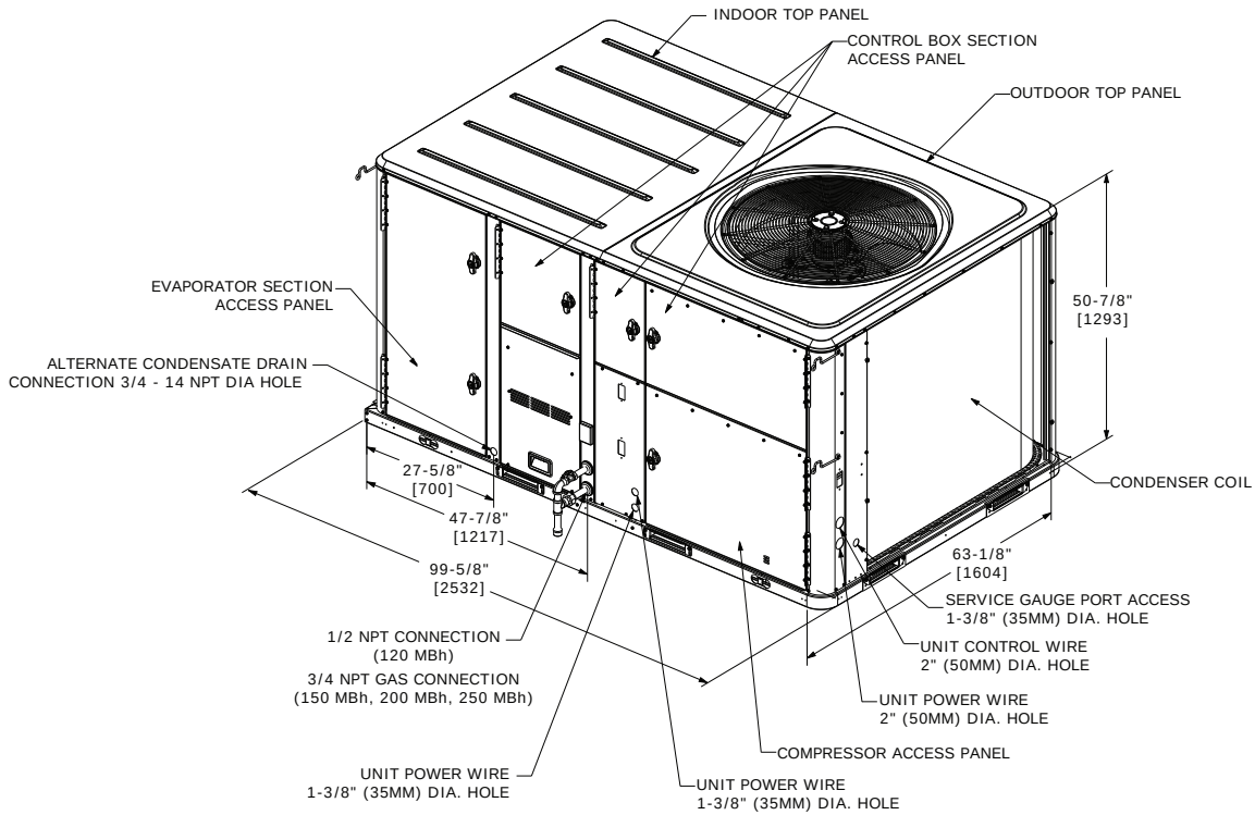
Figure 31. C.O cabinet – downflow airflow supply/return, through-the-base utilities
