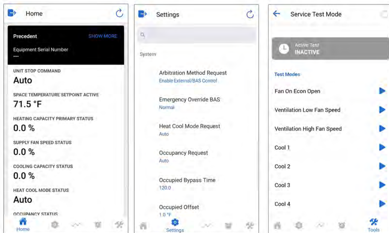
Figure 14. Symbio service and installation mobile app
