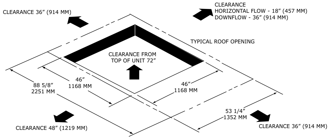
Figure 27. B.O cabinet – roof curb
