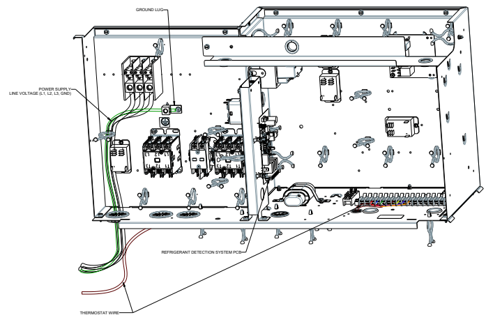
THREE-PHASE FIELD CONNECTIONS
