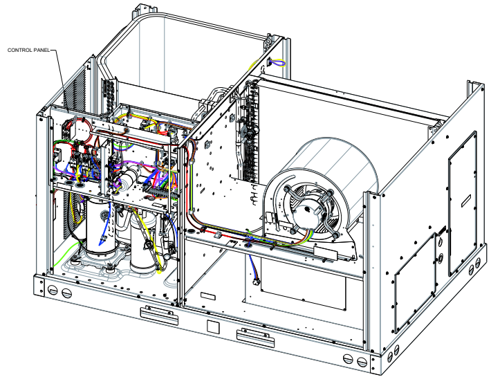
POWER AND LOW VOLTAGE BLOCK CONNECTIONS
