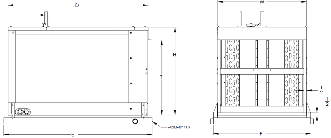
DIMENSIONAL DATA (In.) - FIGURE 1
